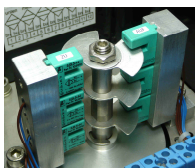
Ex i ... 8 V DC and 24 V DC inductive P+F sensors, Ex eb mb ... / eb db ... 4 - 250 V AC/DC Soldo-Reed switches, Ex 4 - 250 V AC/DC SPDT Bartec switches, 4 - 250 V AC/DC SPDT Crouzet switches
